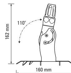
LS679 Pond Monster Mounting Plate Order separately
